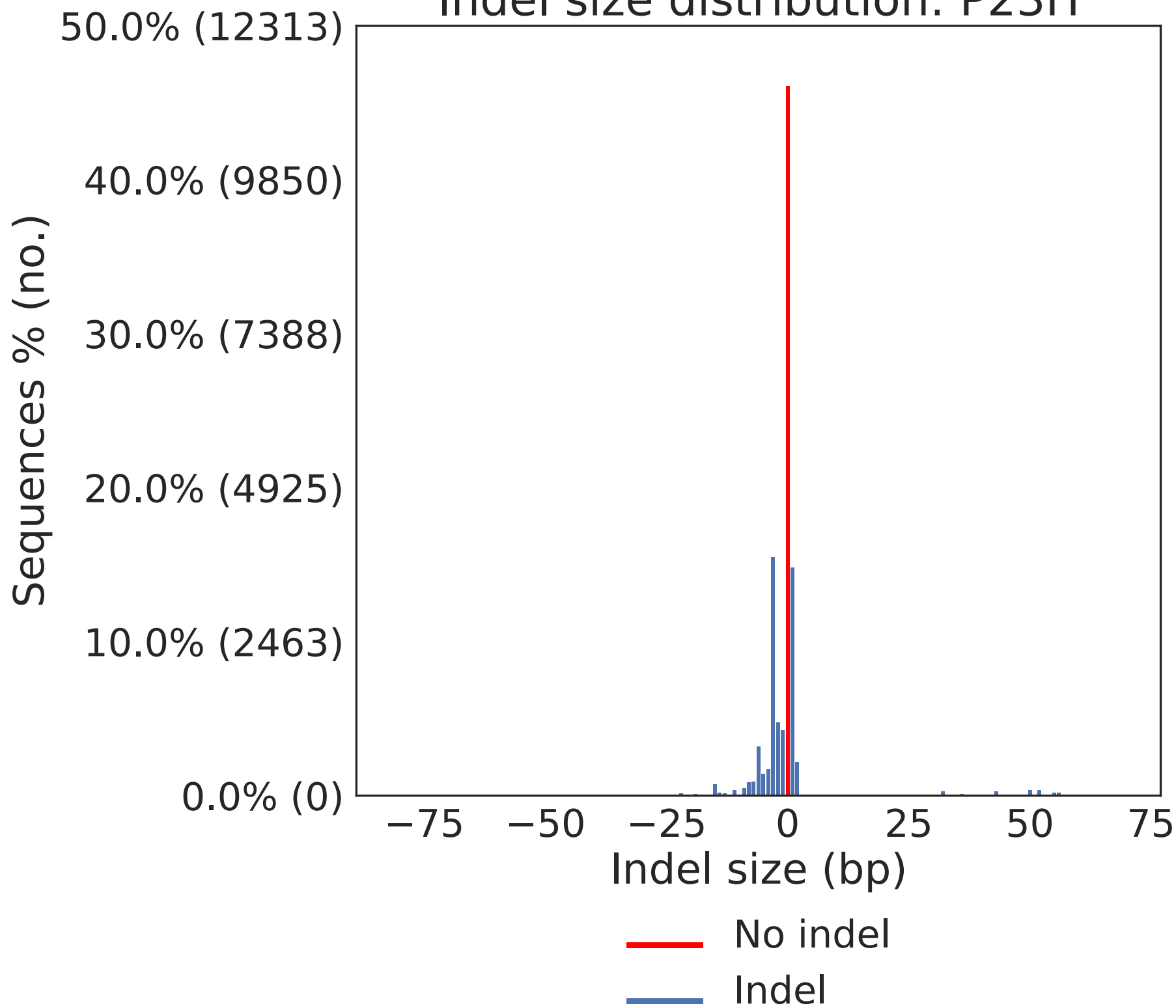
Indel size distribution: P23H
