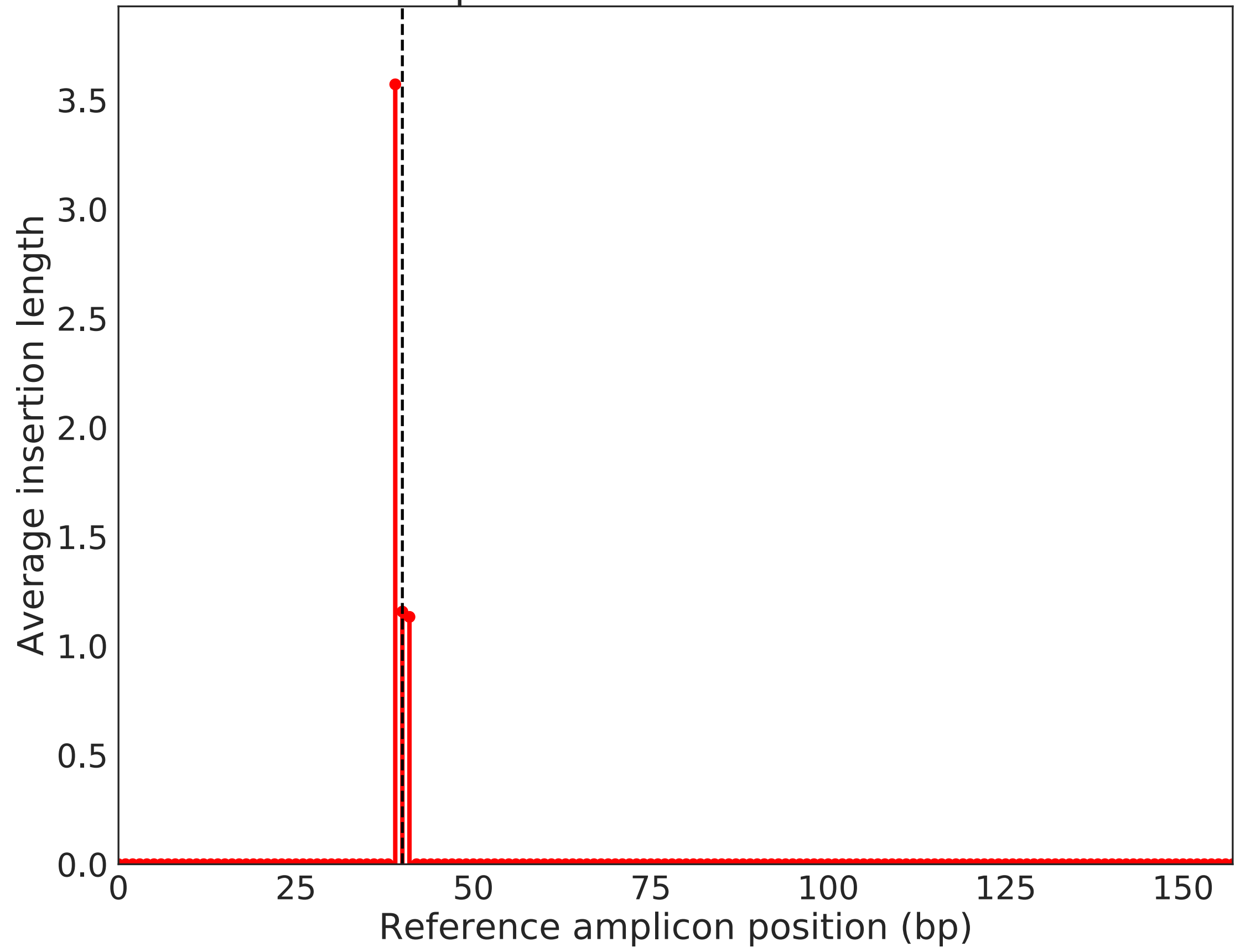
Position dependent insertion size: Reference
