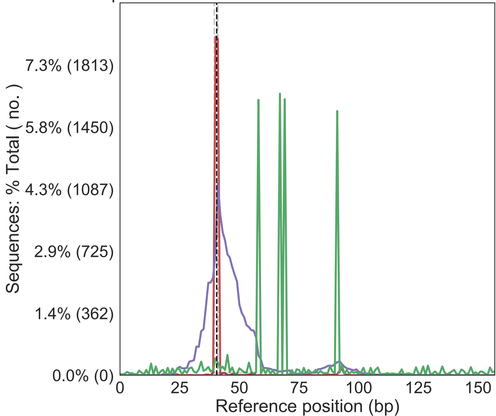
Mutation position distribution in all reads with reference to Reference
